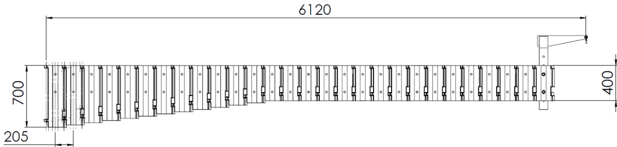
Figure 1: Basic dimensions of JF 100-6.
