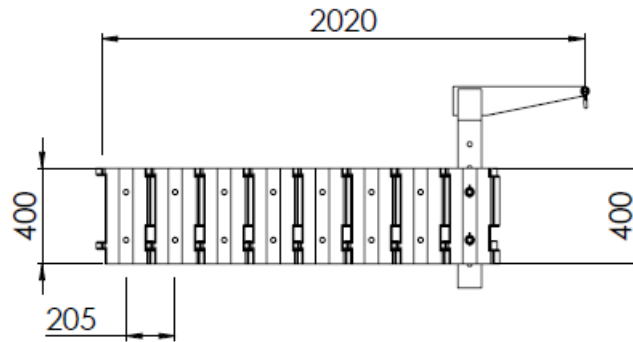
Figure 1: Basic dimensions of JF 150-2.
