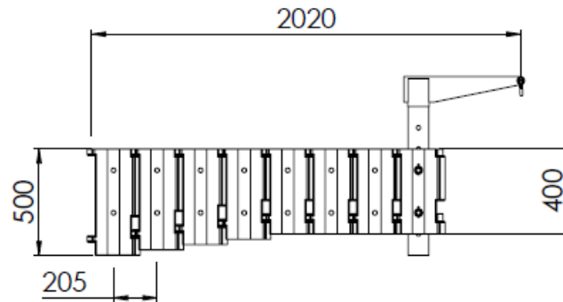
Figure 1: Basic dimensions of JF 350-2.
