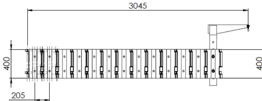
Figure 1: Basic dimensions of JF 50-3.
