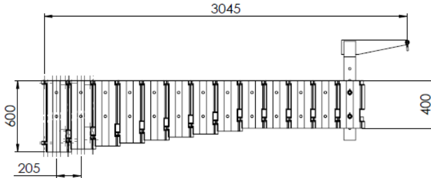
Figure 1: Basic dimensions of JF 300-3.
